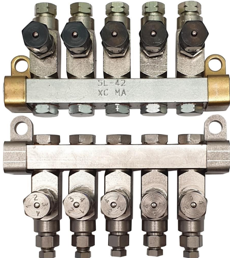
Figure 1. shows 2 typical 5 bank injectors
