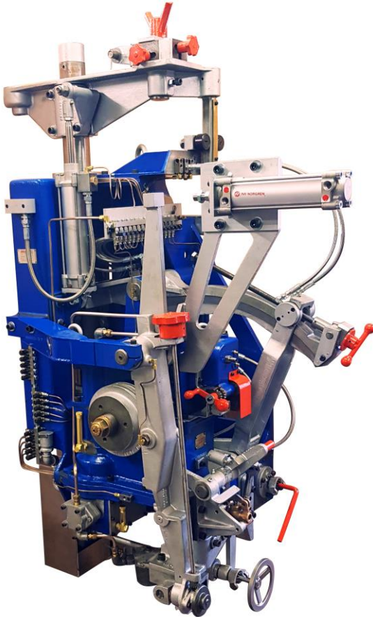
Figure 1. An overhauled 503 10:1 ratio high speed feeder mechanism
