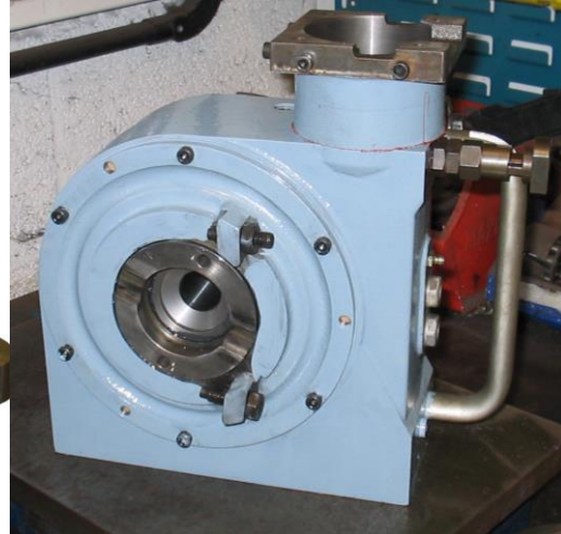
Figure 2. DAO overhauled gearbox ready to ship
